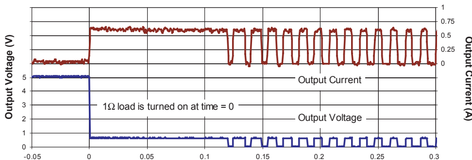
Figure 2: Overload Operation.
